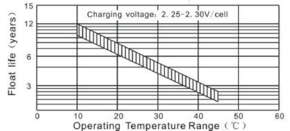
Float service life VS temperature
