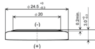
Dimension Drawing
