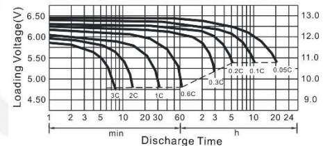
Discharge Characteristics 77°F (25°C)
